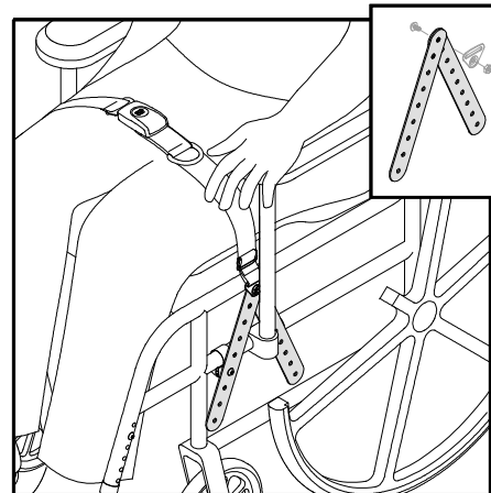
STRAPS SPREAD APART TO SPAN OBSTRUCTIONS
