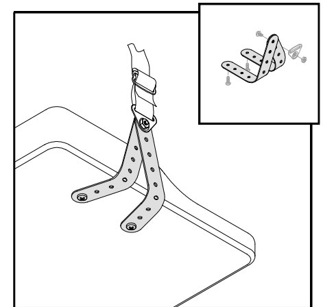
ATTACHED TO SOLID SEAT BOTTOM SCREWS MUST HAVE A MINIMUM PULLOUT STRENGTH OF 90kg (200lbs)
