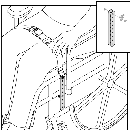
STRAPS ALIGNED TO FIT IN TIGHT SPACES
